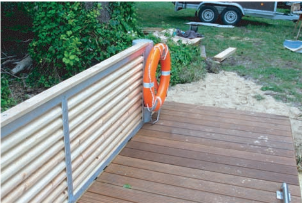
Steganlage, Details
